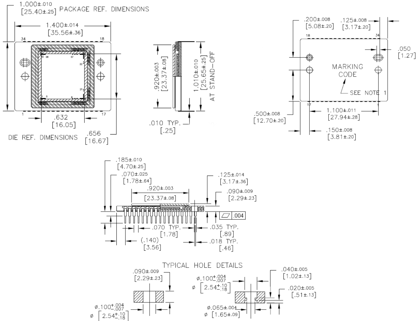
Figure 44: Completed Assembly
